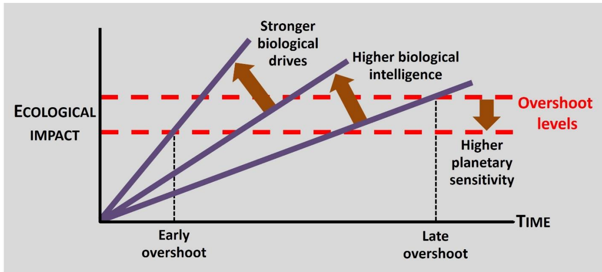
Figure 1-3. Key factors in the timing of ecological overshoot
